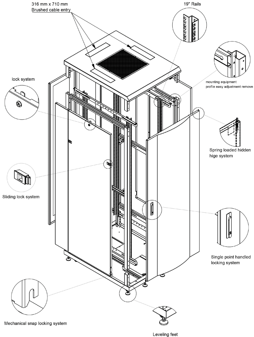
EXPLODED VIEW
